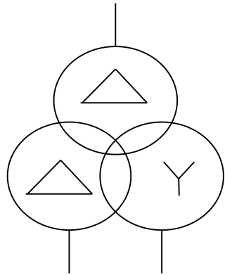
Vilces transformators 10/0,516kV - 1500 kVA
