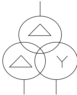
Vilces transformators 10/0,516kV - 1800 kVA
